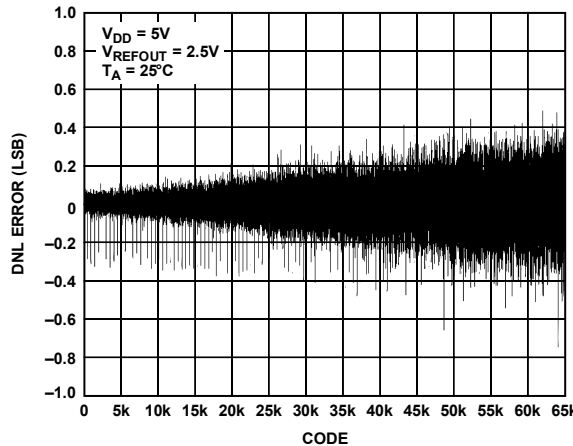
Figure 13. DNL—AD5663R-5
