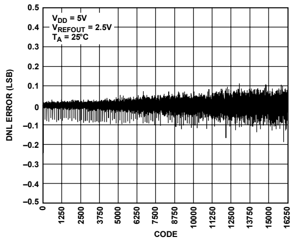
Figure 14. DNL—AD5643R-5
