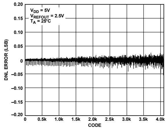
Figure 15. DNL—AD5623R-5
